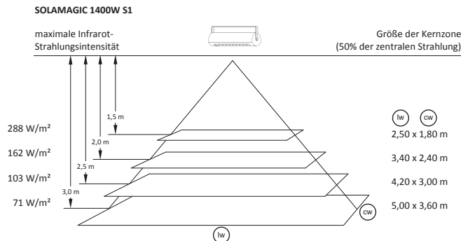
Strahlungspyramide SOLAMAGIC® S1 1400 W
